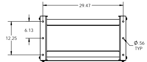
BOTTOM VIEW OPTIONAL SEISMIC MOUNTING FOOTPRINT
