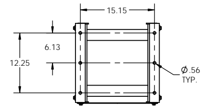
BOTTOM VIEW OPTIONAL SEISMIC MOUNTING FOOTPRINT
