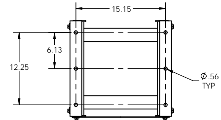
BOTTOM VIEW OPTIONAL SEISMIC MOUNTING FOOTPRINT
