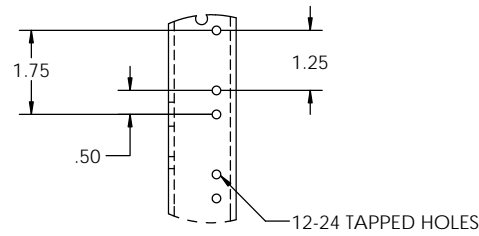
DETAIL A EIA HOLE SPACING
