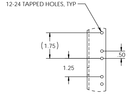
DETAIL A EIA HOLE SPACING
