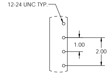
DETAIL C SCALE 1 : 2 WECO HOLE SPACING
