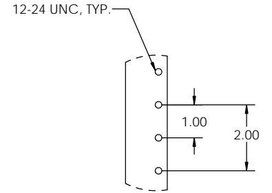
DETAIL D SCALE 1 : 2 WECCO HOLE SPACING
